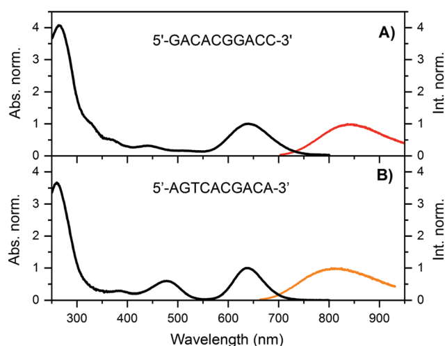
Fig. 1 Normalized absorption (at the 640 nm transition, T = 25\text{ }^{\circ}\text{C} ) and emission spectra (recorded at room temperature on a single molecule sensitive confocal microscope) 12 for (A) DNA841-AgNCs and (B) DNA811-AgNCs in a 10 mM ammonium acetate ( \text{NH}_4\text{OAc} ), exciting at 640 and 645 nm, respectively.
