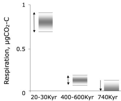
Fig. 4. Respiration in micrograms of CO 2 -C per gram of dry soil per day as a function of permafrost age; the range depicted represents the minimum detectable difference by this method.
